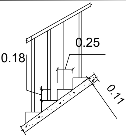
STAIRCASE DETAILS:-
