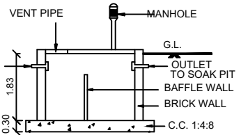
SECTION OF SEP.TANK
