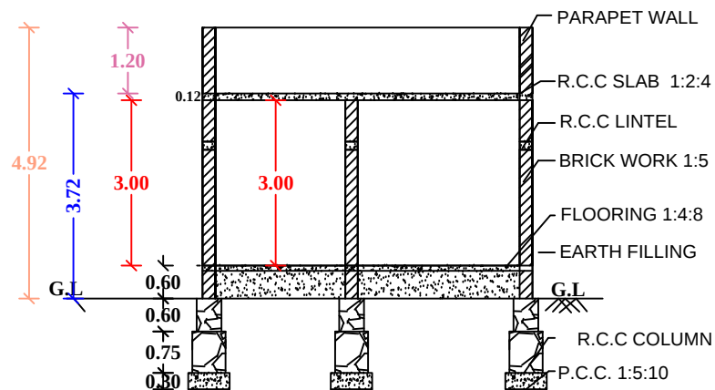
"SECTION "AB"
