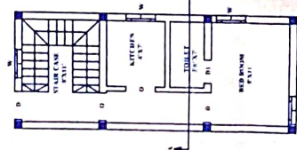
FIRST FLOOR PLAN - WEST FACING
