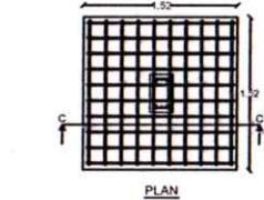
COLOUMN FOUNDATION DETAILS
