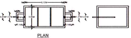
PLAN & SECTION OF SEPTIC TANK & DISPERSION TRENCH
