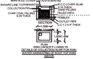
DETAILS OF COLLECTION RUMP FOR RAIN WATER
