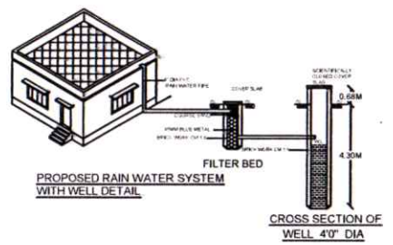
DETAILS OF COLLECTION RUMP FOR RAIN WATER
