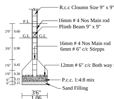
COLUMN DETAIL
