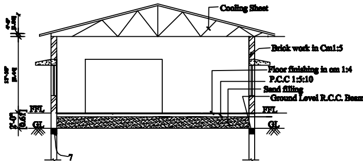
FOUNDATION DETAIL DESIGNED AS PER LOCAL SOIL CONDITION SECTION ON "JS"
