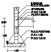
COLUMN DETAILS Size of column = 0.25m x 0.25m Not to scale
