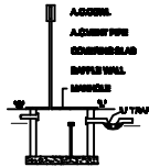
SEPTIC TANK DETAILS
