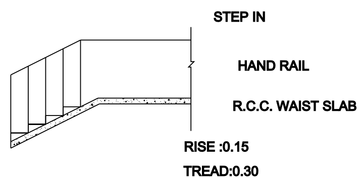
STAIR DETAILS
