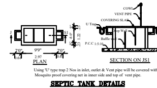
SEPTIC TANK DETAILS
