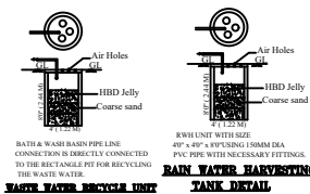
RAIN WATER HARVESTING TANK DETAIL
