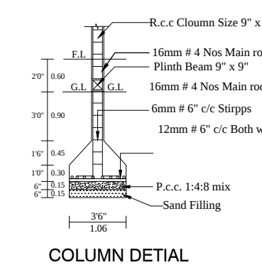
COLUMN DETAIL
