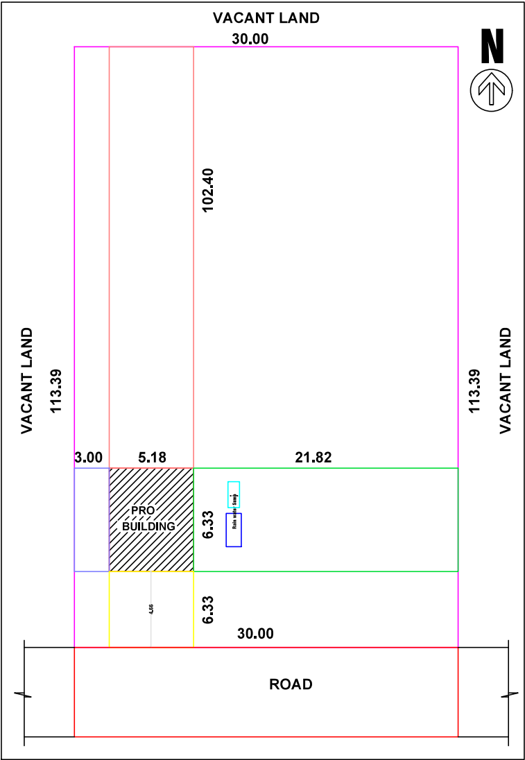
SITE PLAN & KEY PLAN
