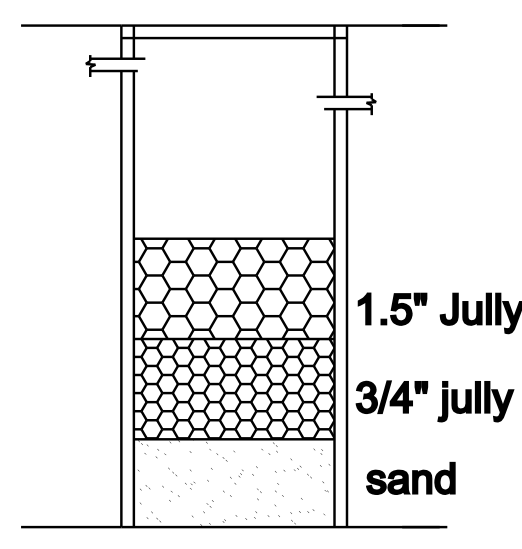
RAIN WATER HARVESTING TANK
