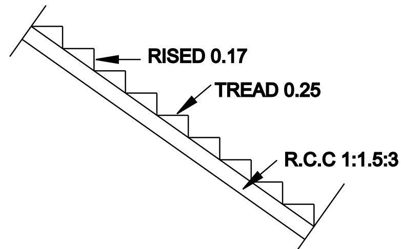
STAIRCASE DETAILS
