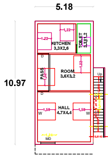
GROUND FLOOR I
