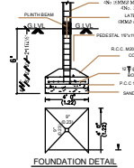
FOUNDATION DETAIL
