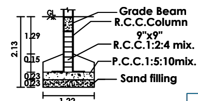
COLUMN DETAILS
