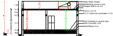
SECTION - "AB "
