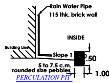
RAIN WATER PIPE
