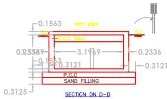
SECTION ON D-D
