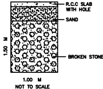
RAIN WATER HARVEST COLLECTION PIT.
