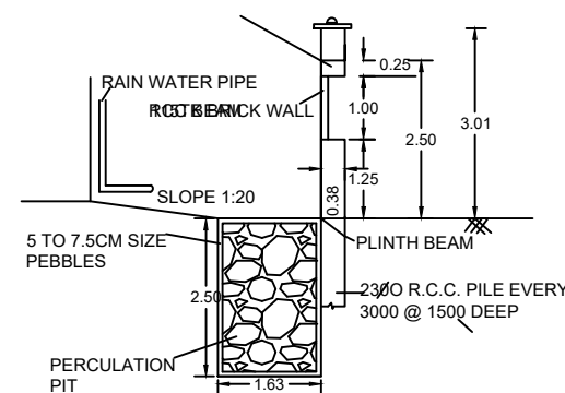
RAINWATER HARVESTING
