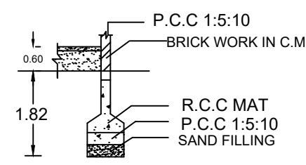
FOUNDATION DETAILS
