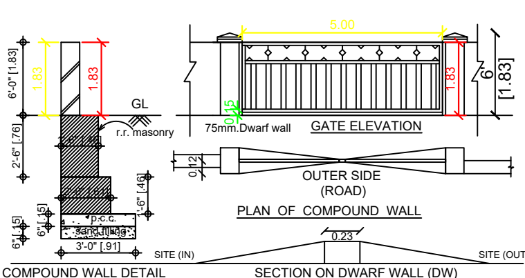
COMPOUND WALL DETAIL
