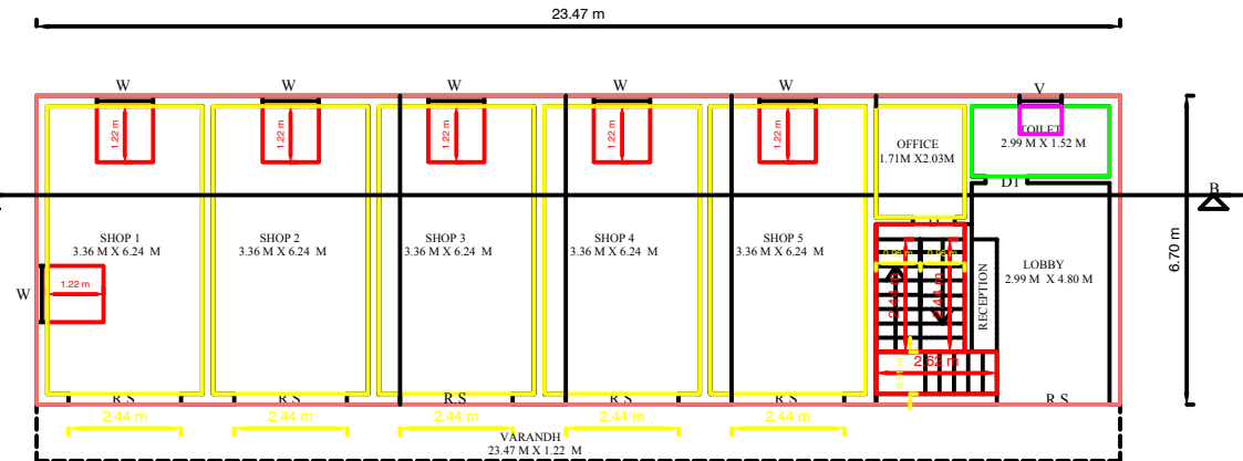
COMMERCIAL - PLAN
