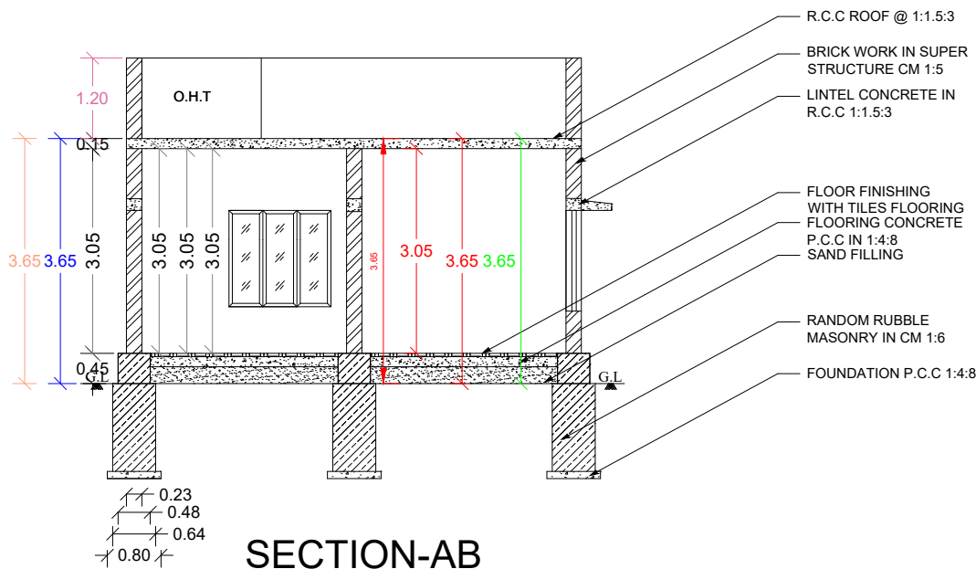
SECTION-AB
