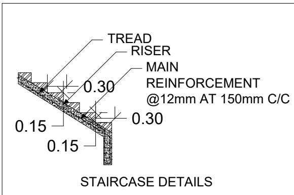
STAIRCASE DETAILS
