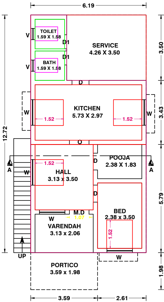
EXI & PRO.GROUND FLOOR PLAN
