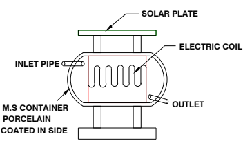
SOLAR SYSTEM
