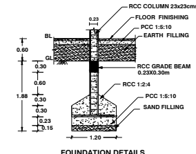
FOUNDATION DETAILS
