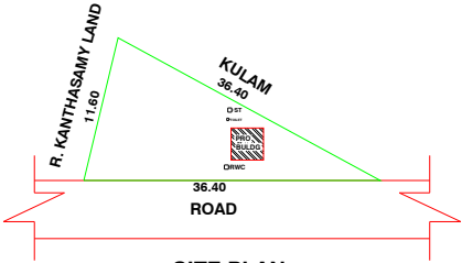
SITE PLAN (NOT TO SCALE)
