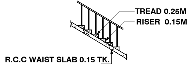
STAIR CASE DETAILS
