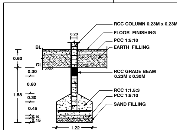
FOUNDATION DETAILS
