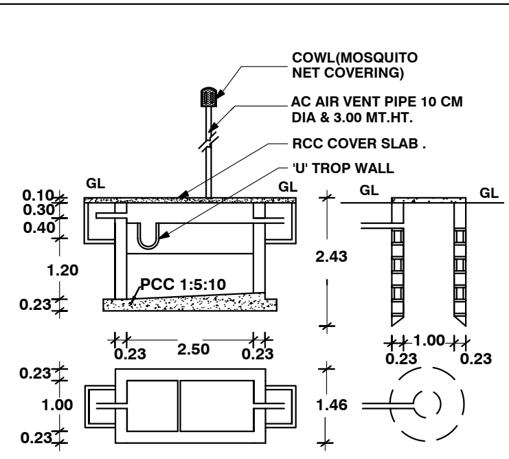
PLAN AND CROSS SECTION OF ST & SP.
