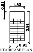
STAIRCASE PLAN
