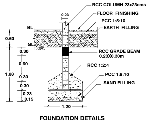
FOUNDATION DETAILS
