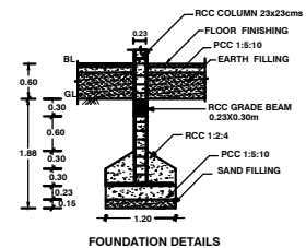
FOUNDATION DETAILS
