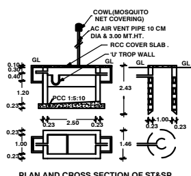
PLAN AND CROSS SECTION OF ST&SP.
