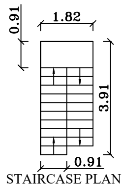
STAIRCASE PLAN
