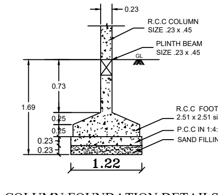
COLUMN FOUNDATION DETAILS
