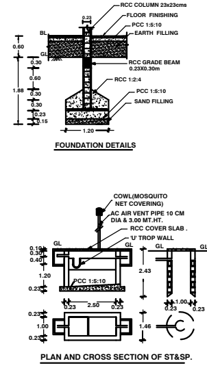
FOUNDATION DETAILS
