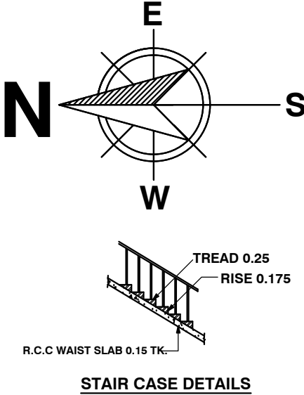
STAIR CASE DETAILS
