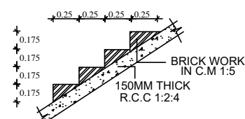
STAIRCASE DETAILS
