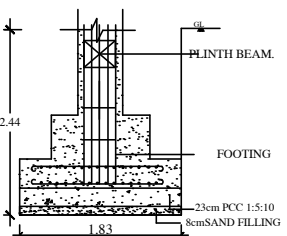
COLUMN FOUNDATION DETAILS
