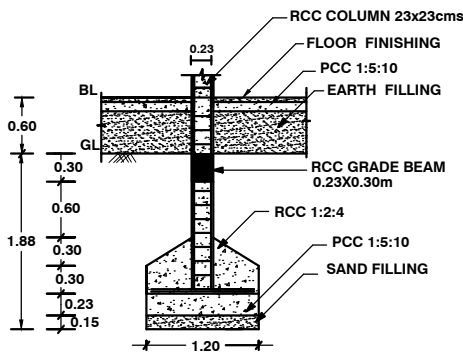
FOUNDATION DETAILS
