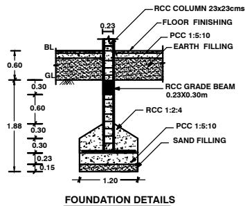
FOUNDATION DETAILS
