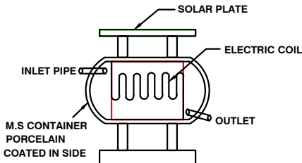
SOLAR SYSTEM
