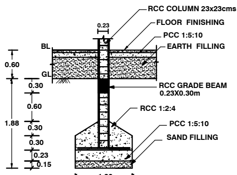
FOUNDATION DETAILS
