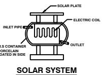
SOLAR SYSTEM
