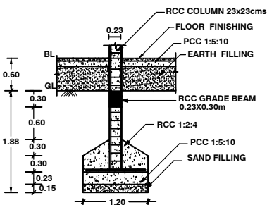
FOUNDATION DETAILS
