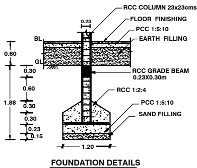
FOUNDATION DETAILS
