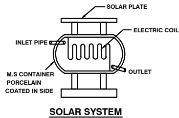
SOLAR SYSTEM
