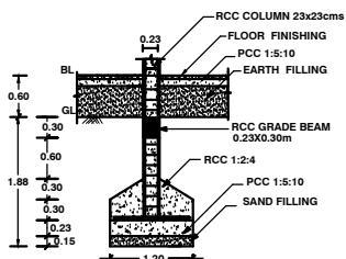
FOUNDATION DETAILS
