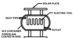
SOLAR SYSTEM
