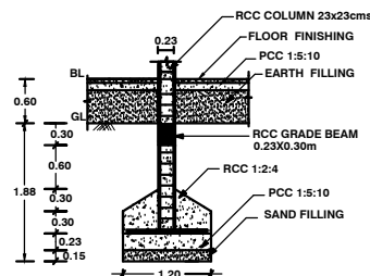
FOUNDATION DETAILS
