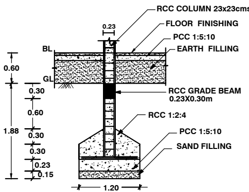
FOUNDATION DETAILS
