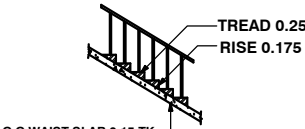
STAIR CASE DETAILS
