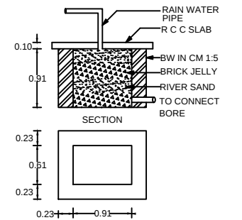
RAIN WATER COLLECTION TANK
