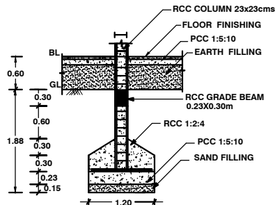
FOUNDATION DETAILS
