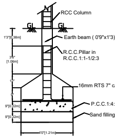
FOUNDATION DETAILS
