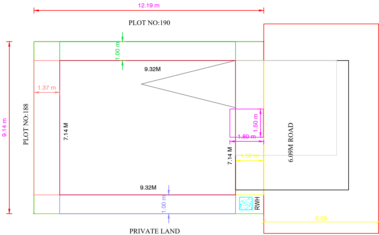
SITE PLAN
