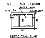
SEPTIC TANK PLAN
