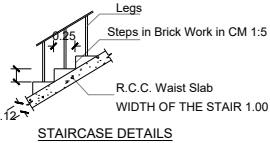
STAIRCASE DETAILS
