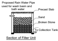
Section of Filter Unit
