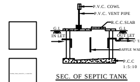
SEC. OF SEPTIC TANK
