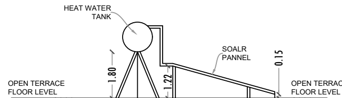
SIDE ELEVATION
