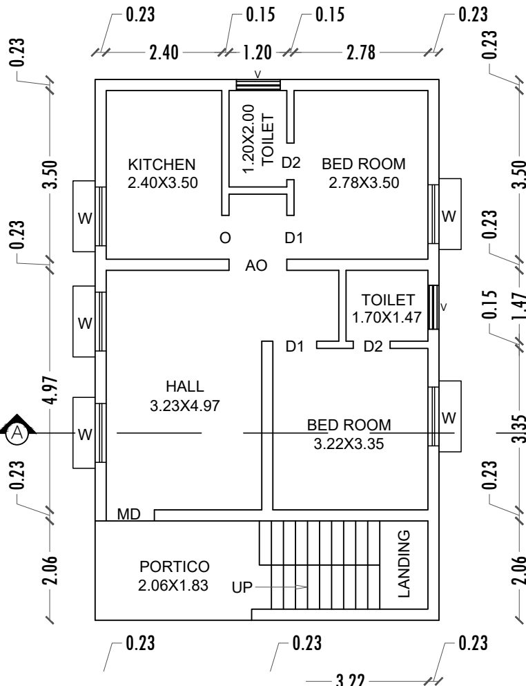
GR PLAN
