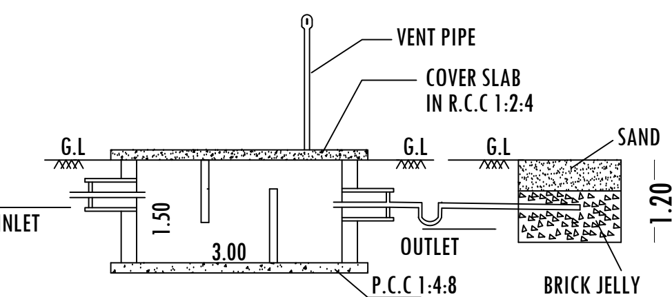
SECTION-AB
