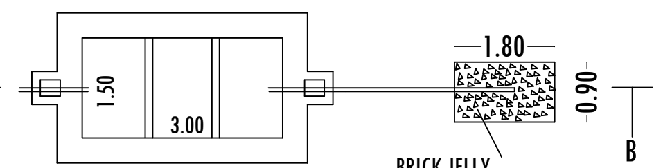
SEPTIC TANK & DISPERSION TRENCH DETAILS
