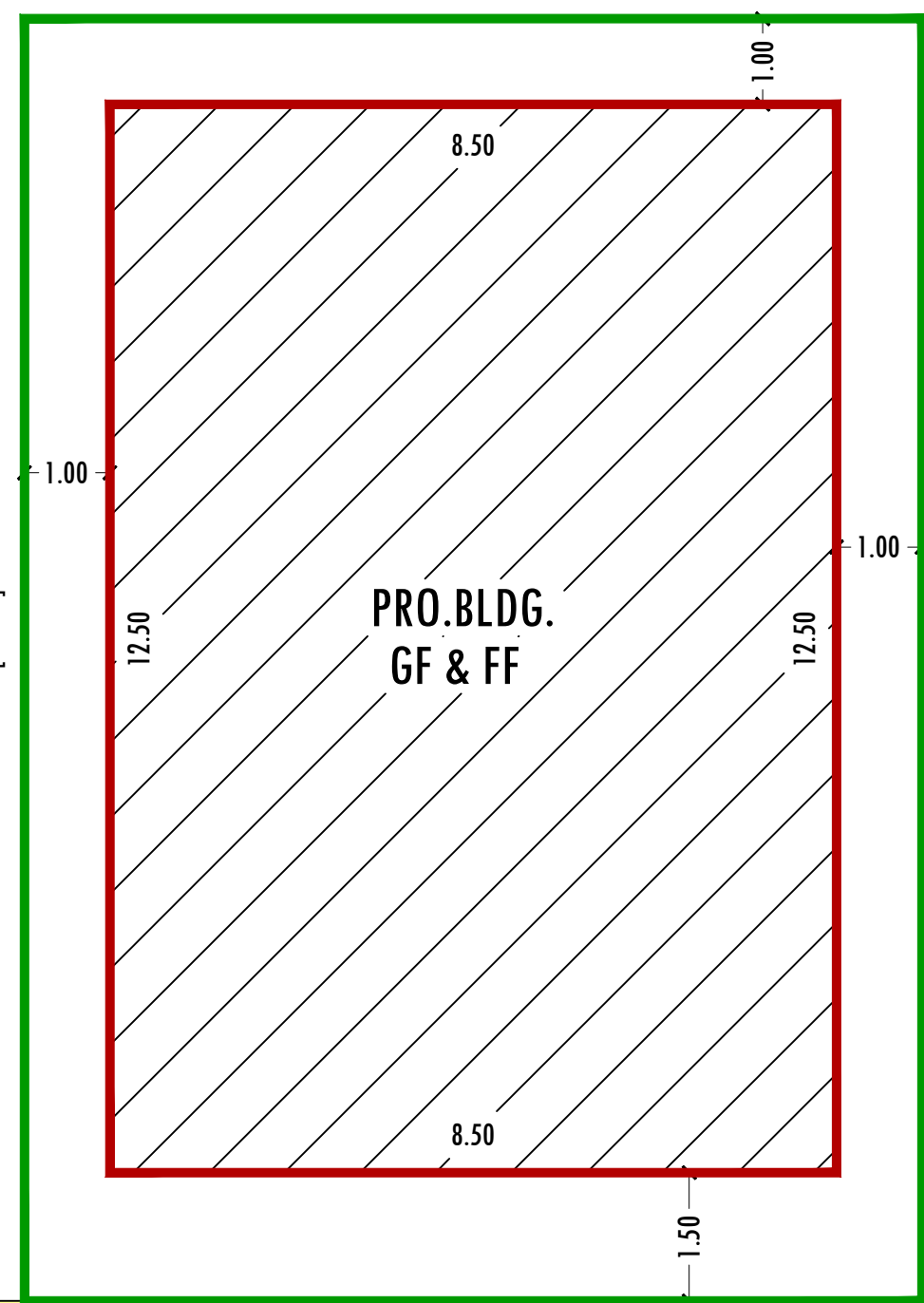
9.00 M ROAD
