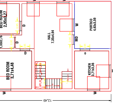
PRO., GROUND FLOOR PLAN
