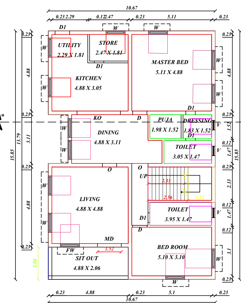
FLOOR - GROUND PRO. GROUND FLOOR PLAN
