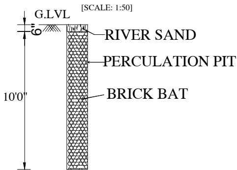
PERCOLATION PIT
